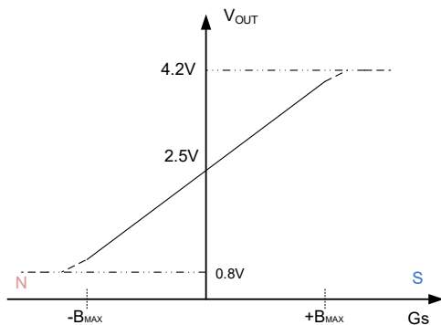
Fig 5-1. T092S PKG Output-5V
