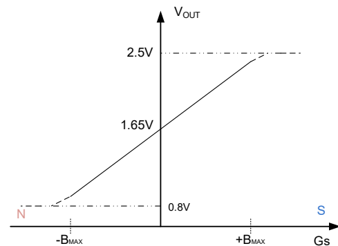
Fig 5-2. T092S PKG Output-3.3V
