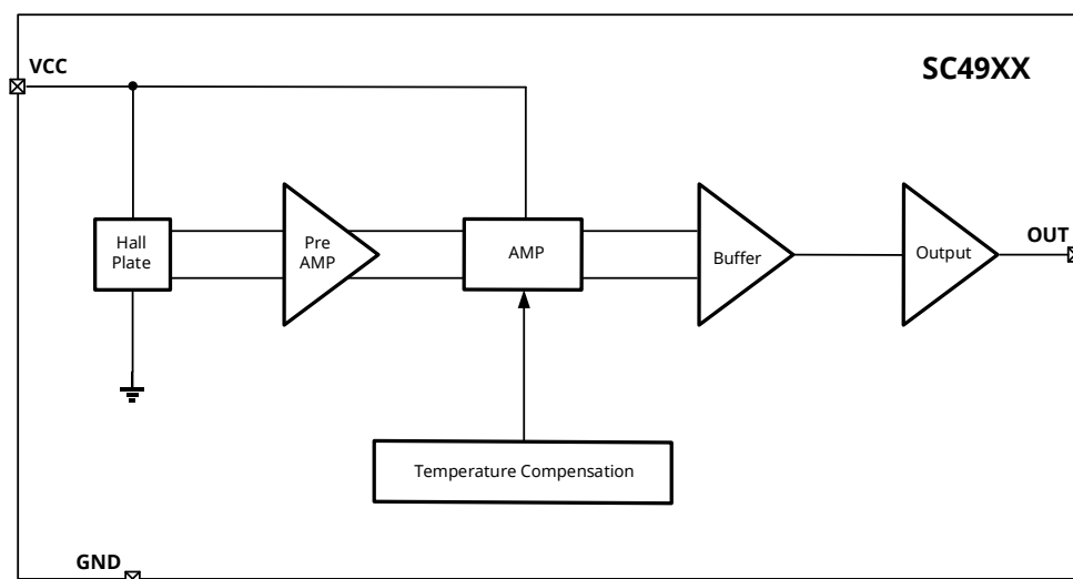
Fig.3 Block Diagram
