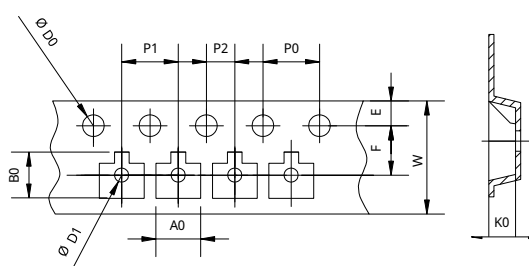
TAPE DIMENSIONS
