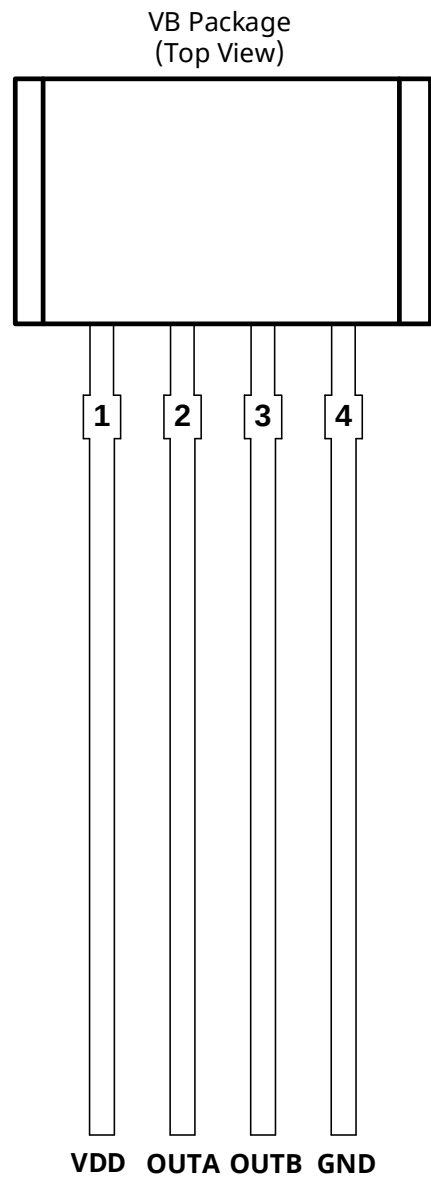
Fig.2 Pin Description
