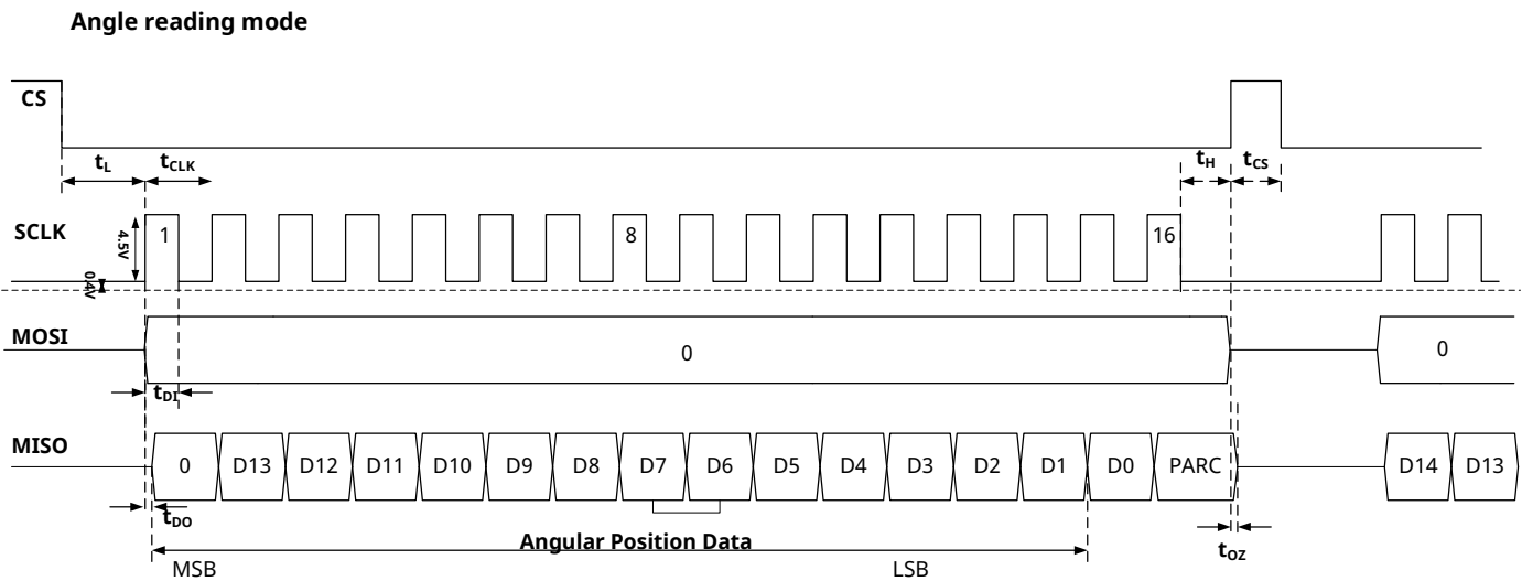
Fig.9 SPI angle reading mode diagram
