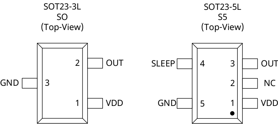
Fig.2SOT23-3L(Left) and SOT23-5L(Right)Pin Description
